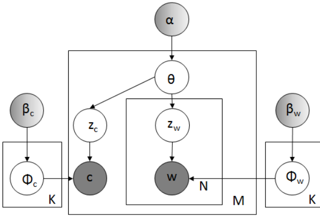
Figure 3: Plate notation of our LDA variant. Categories and words are respectively denoted as c and w . Gradient colored nodes are time-dependent parameters.
