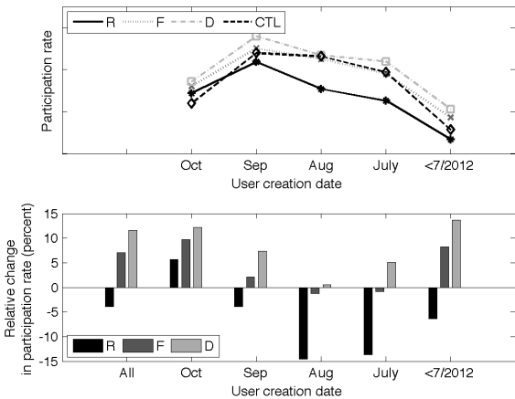
Figure 7: Answering participation rate over time
