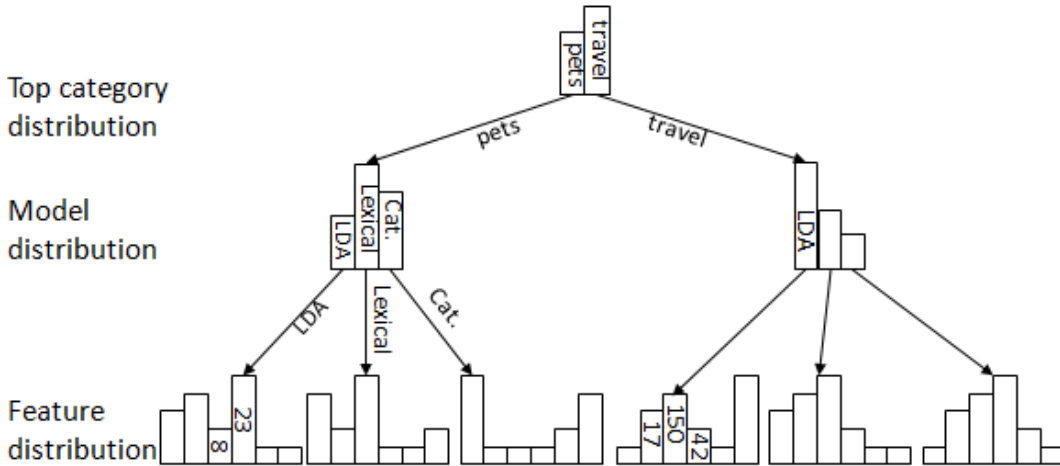
Figure 4: User profile as a probability distribution tree
